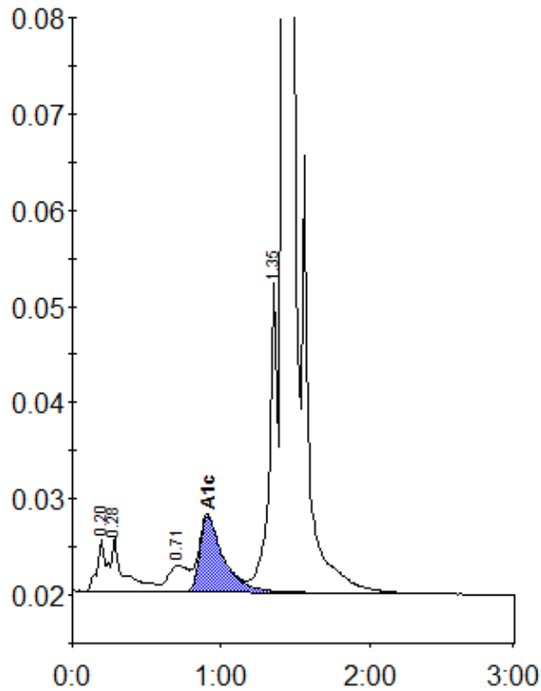
Peak table - ID: 10563989
